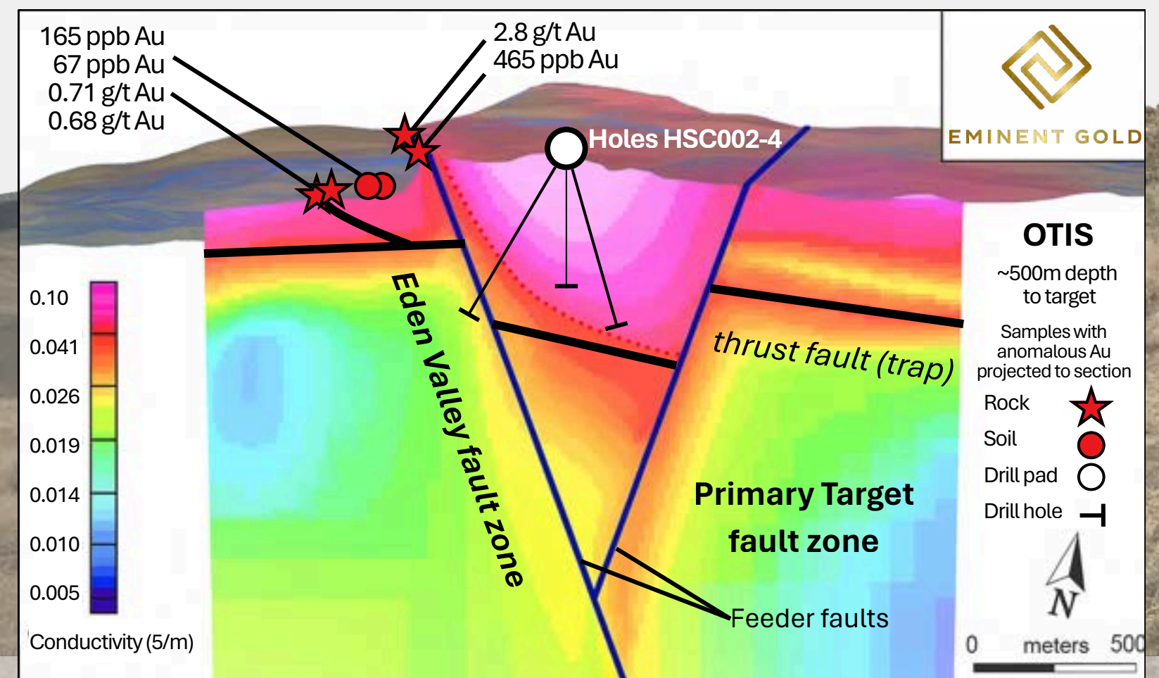
Magnified CSAMT cross-section: looking north
