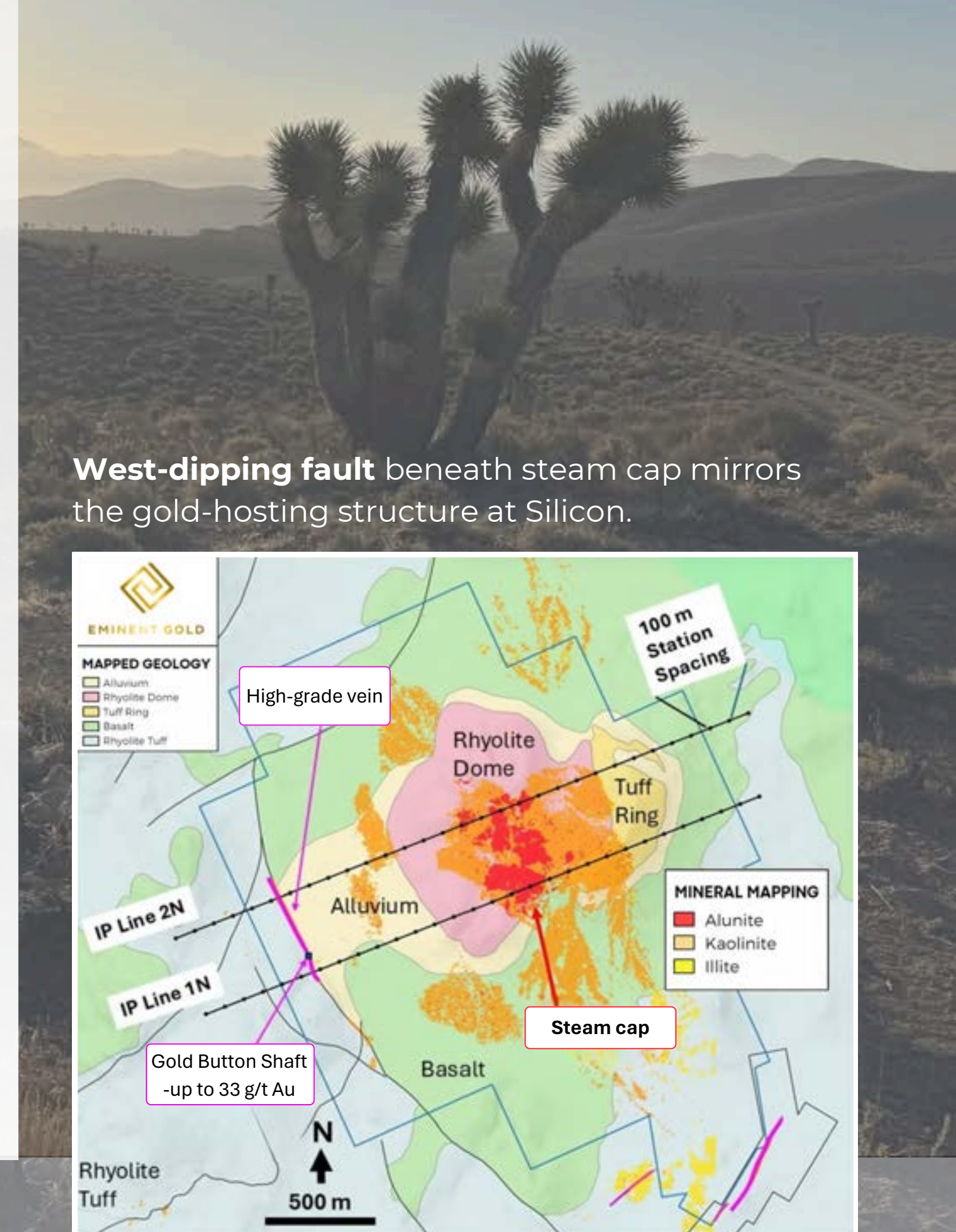
Geophysical/section lines on geology, alteration, showing major structure
