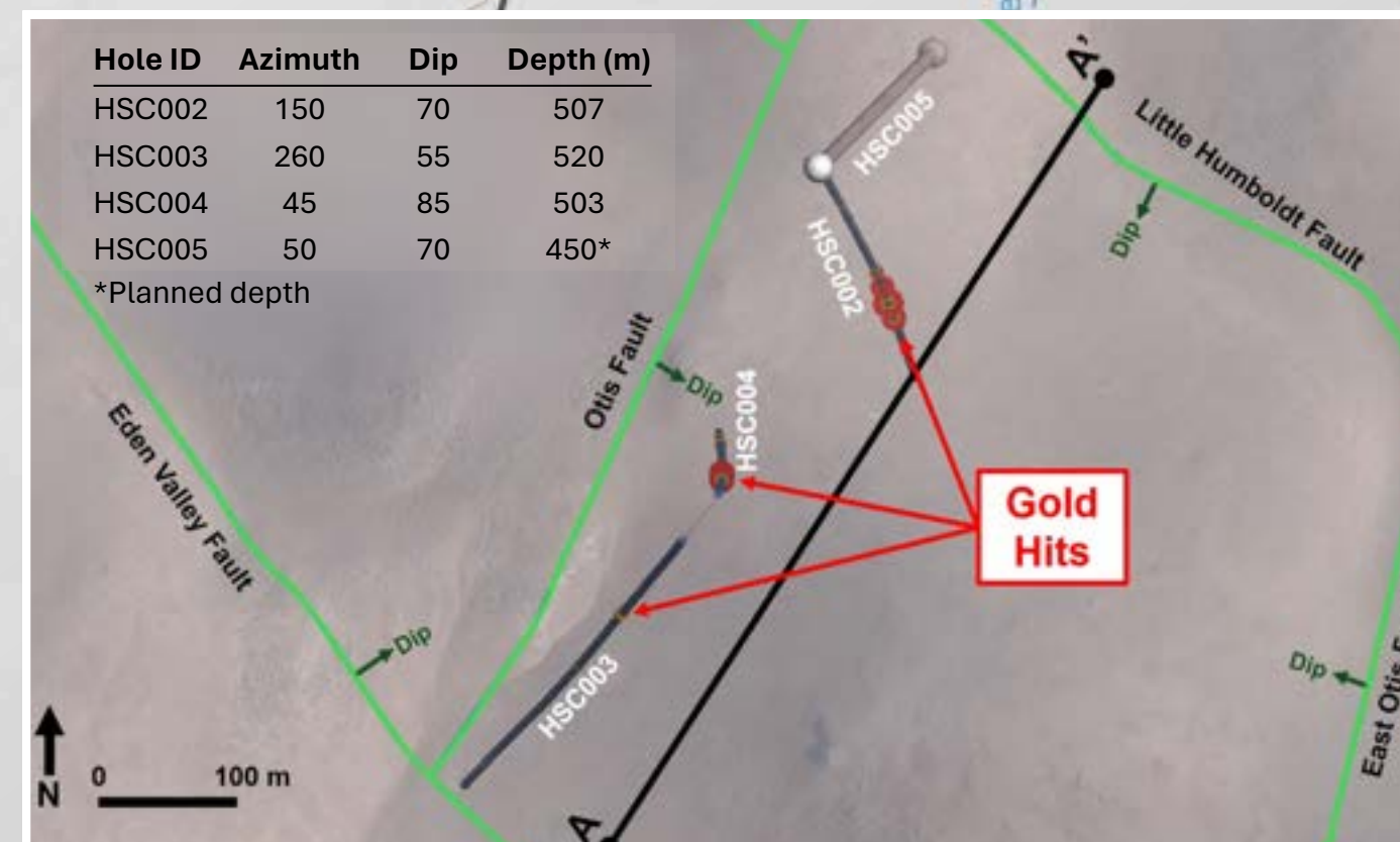
Otis Target drill layout: completed and planned holes over fault map
