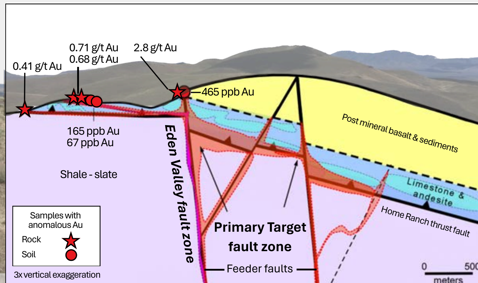
Interpreted geological cross-section: looking north
