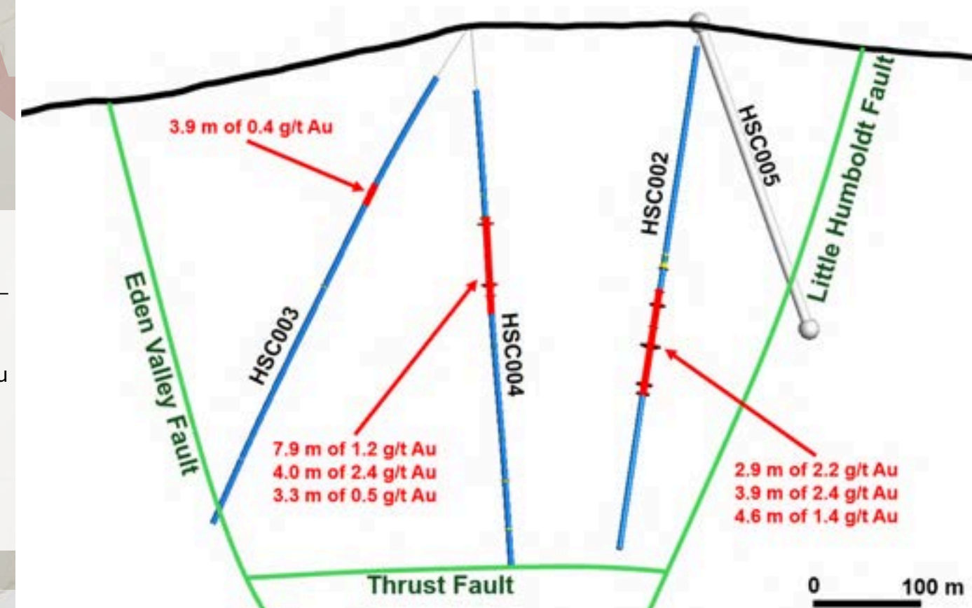
Cross Section A-A' Looking Northwest
